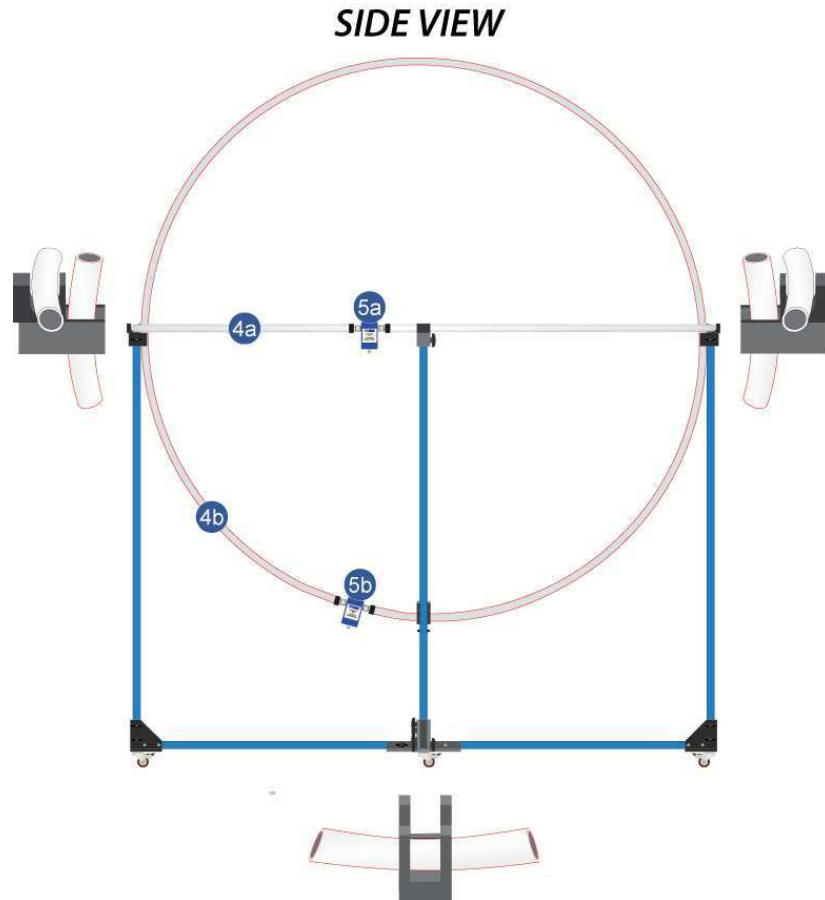
Figure 13 – ALT-930-2M Triple Loop Antenna Assembly – Step #9
