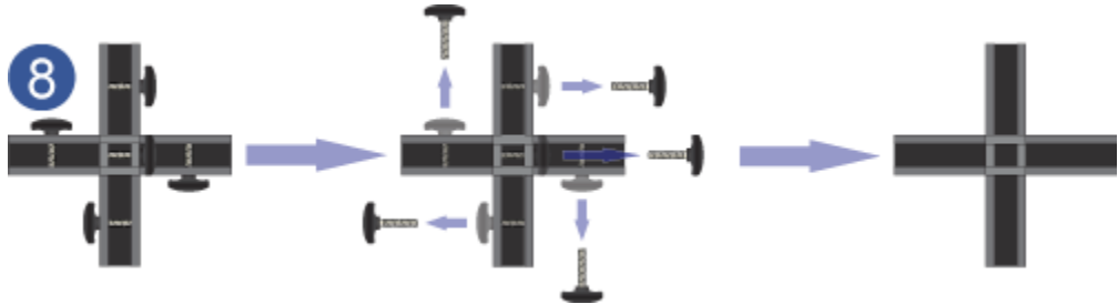
Figure 5 - ALT-930-2M Triple Loop Antenna Assembly – Step #1
